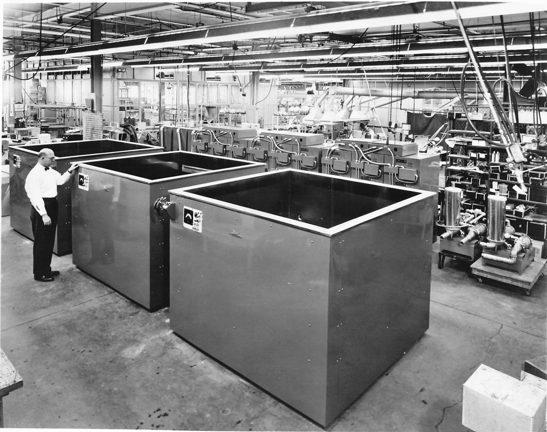
Bendix Sonic Energy Cleaners 72" x 75" x 48" deep
